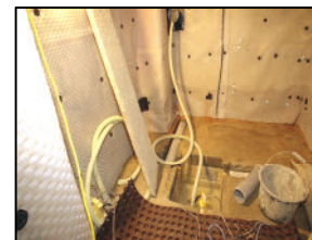
Sump and pumps installed and ready for test
